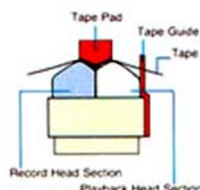
Figure 8 Closeup View Of Head Contact Area
