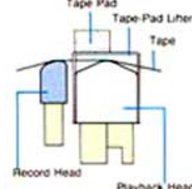
Figure 8 Closeup View Of Head Contact Area
