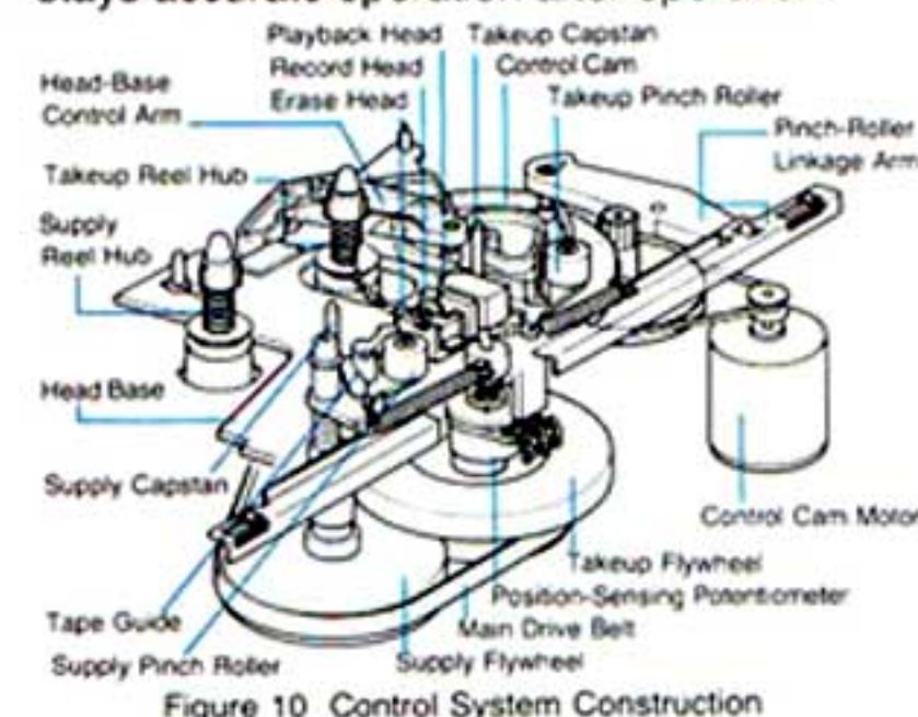
Figure 10 Control System Construction
