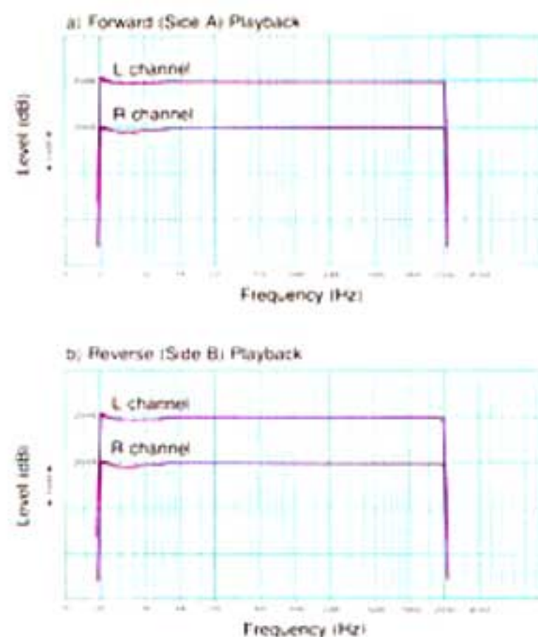
Figure 3 Frequency Response
